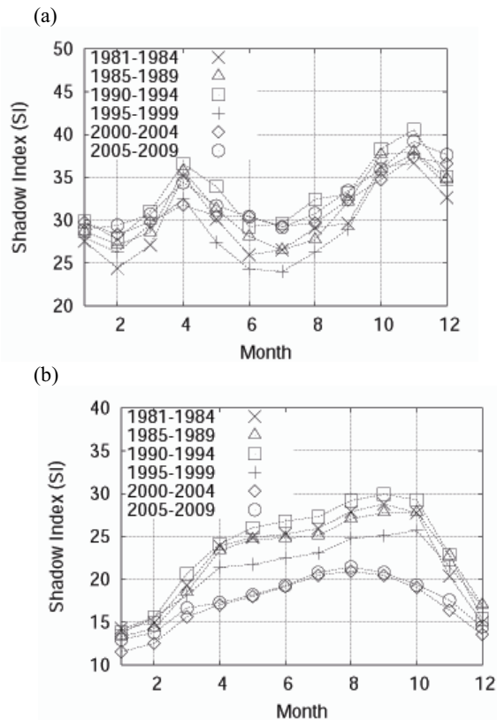
Figure 2. The seasonal change of Shadow Index (SI) in (a) Japan and (b) Mongolia. Used SI values are mean value of five years data, which were observed by NOAA/AVHRR and Terra/MODIS from 1981 to 2009.
