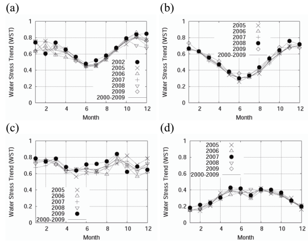
Figure 4. The seasonal change of Water Stress Trend (WST) in (a) Australia, (b) Argentina, (c) Kenya, and (d) Japan. Used data were observed by Terra/MODIS from 2000 to 2009.
