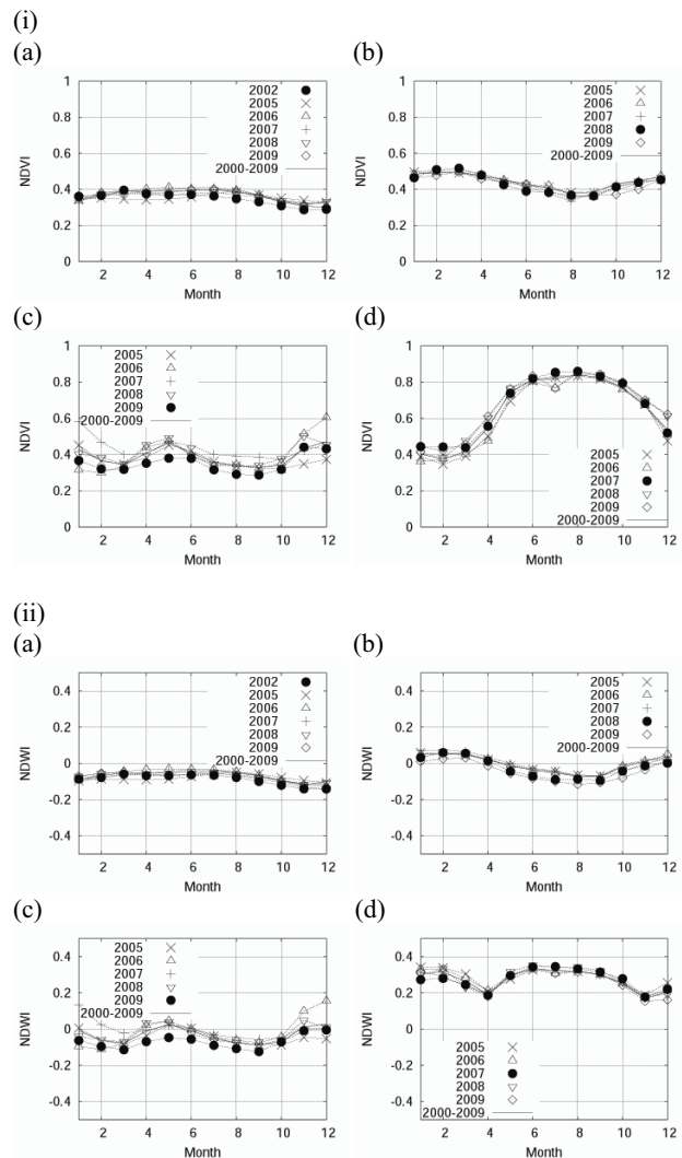
Figure 5. The seasonal change of (i) NDVI (Normalized Difference Vegetation Index), and (ii) NDWI (Normalized Difference Water Index) in (a) Australia, (b) Argentina, (c) Kenya, and (d) Japan. Used data were observed by Terra/MODIS from 2000 to 2009.
