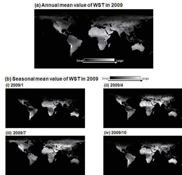
Figure 3. The global images are (a) annual mean value and (b) seasonal mean value of Water Stress Trend (WST). Used data were observed by Terra/MODIS in 2009.
