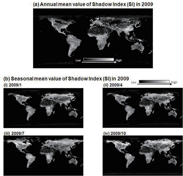
Figure 1. The global images are (a) annual mean value and (b) seasonal mean value of Shadow Index (SI). Used data were observed by Terra/MODIS in 2009.
